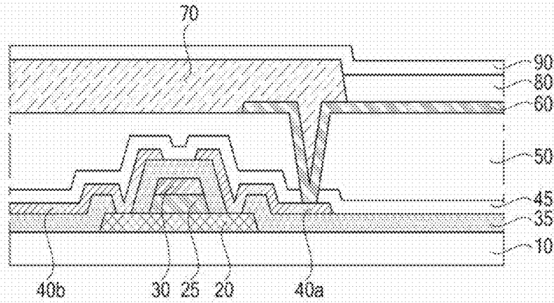
FIG. 1 (Related Art)
